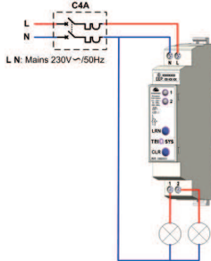
Schematic diagram of electrical connection to lighting loads. They can be replaced by other types of loads (see table §3).
